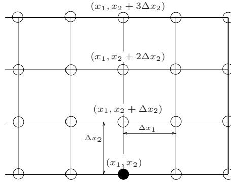
Figure B.1: Schematic of mesh indicating a boundary node at the bottom boundary of a beam
