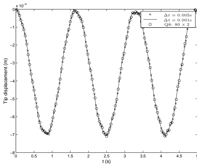
Figure 4.13: Transient response of a cantilever beam when a shear traction of 0.1 Pa is suddenly applied at the free end: (a) Q8 40 \times 1 mesh; (b) using different timesteps and mesh sizes
